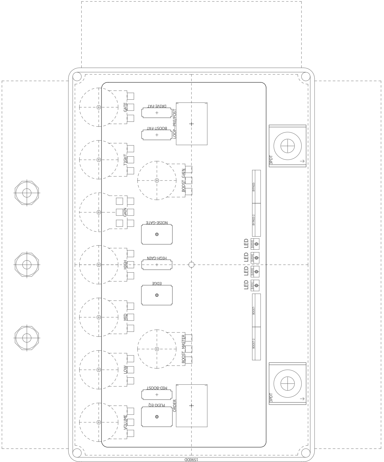
Solid Metal Pro 1590DD enclosure Ready to print A4 page
